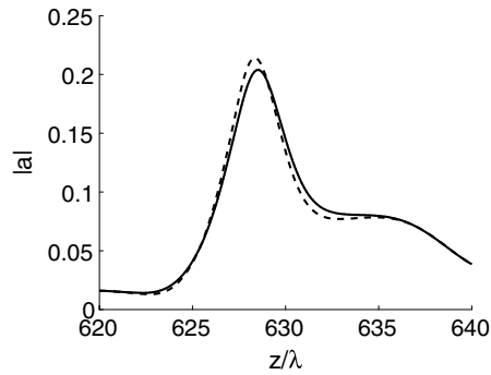
Fig. 7. Results of simulations using the two-level approach compared to a one-level simulation on the (same) coarse grid only. Solid: reference solution, dashed: solution computed on a coarse grid only, dotted: two-level approach (curve coincides with the solid one).
