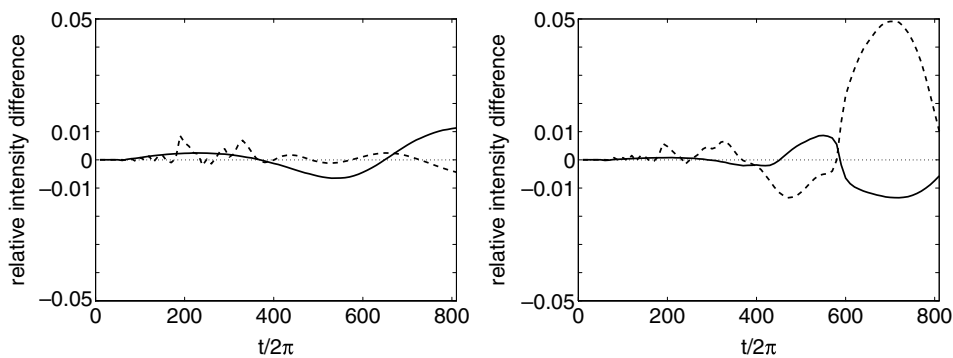
Fig. 8. Relative difference in intensity to the reference solution of the reduced model for a_0 = 0.1 (left) and a_0 = 0.12 (right). Gautschi + QEA (see Table 1, solid) and PIC (dashed) with N = 2 \times 10^5 , \tau = dz(N) and 3 particles per cell, runtime around 5:30 h.
