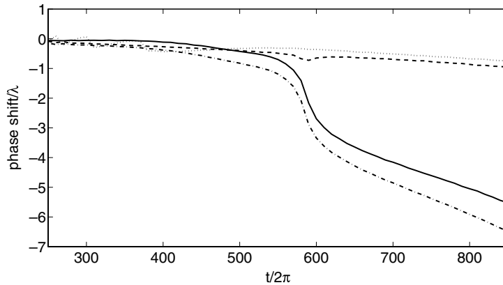
Fig. 10. Phase-difference to the exact linear solution for PIC ( a_0 = 0.12 : dash-dotted and a_0 = 0.0001 : dotted) and Gautschi + QEA ( a_0 = 0.12 , solid), difference between PIC and Gautschi + QEA for a_0 = 0.12 (dashed).
