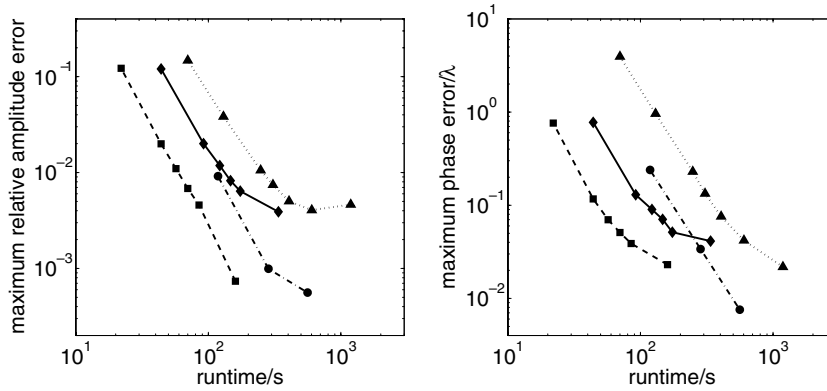
Fig. 4. Same as Fig. 3, but for a_0 = 0.12 .
