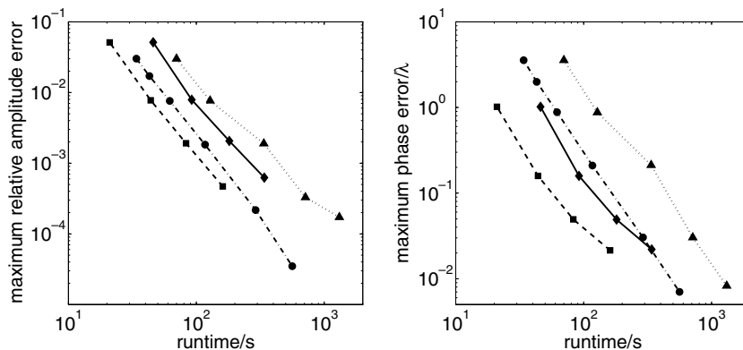
Fig. 3. Maximum amplitude and phase error vs. runtime ( a_0 = 0.1 ) for varying \tau for leap-frog (dotted + triangles), Gautschi (solid + diamonds), leap-frog + QEA (dash-dotted + circles) and Gautschi + QEA (dashed + squares). We used N = 2^{12} for methods without QEA and N = 2^{11} for methods with QEA (see also Table 1).
